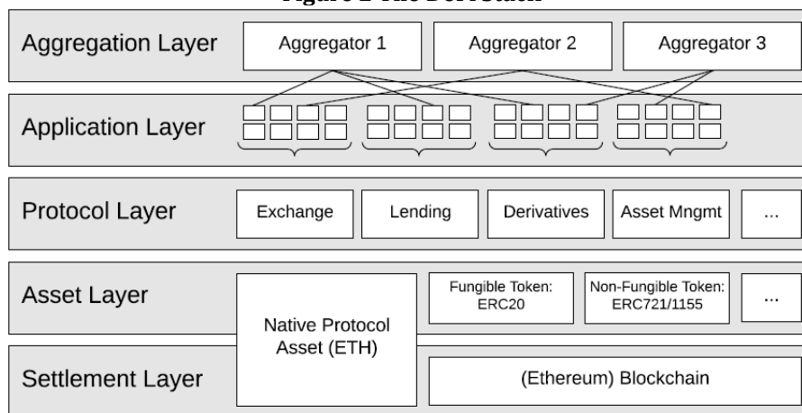
Figure 2 The DeFi Stack
