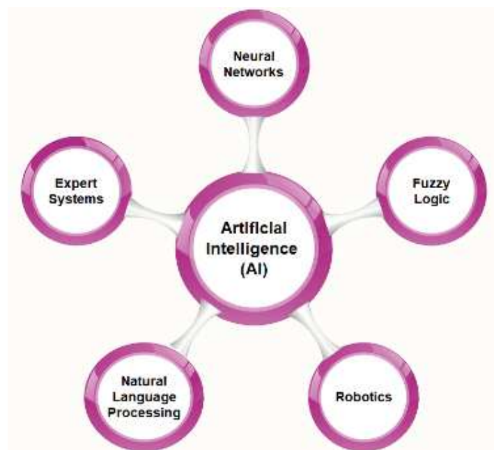
Figure 2 AI tools.
